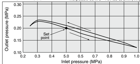
ARM5AA1-308-1 Condition: Inlet pressure 0.5 MPa Outlet pressure 0.2 MPa Flow rate 20 L/min (ANR)
