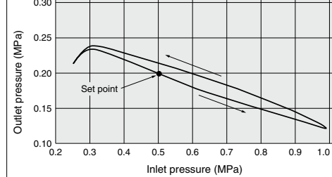
ARM5SA-08-1 Condition: Inlet pressure 0.5 MPa Outlet pressure 0.2 MPa Flow rate 20 L/min (ANR)
