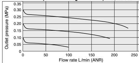
ARM5AA1-309-1 (One-touch fittings: IN \phi 8, OUT \phi 4) Condition: Inlet pressure 0.5 MPa
