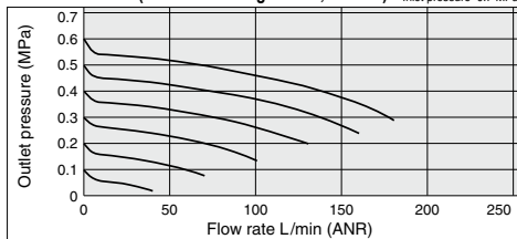
ARM5AA1-310 (One-touch fittings: IN \phi 8, OUT \phi 6) Condition: Inlet pressure 0.7 MPa
