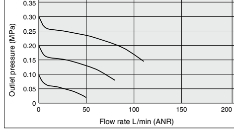
ARM5SA-07-1 (One-touch fittings: IN \phi 6 , OUT \phi 4 ) Condition: Inlet pressure 0.5 MPa
