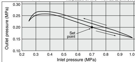
ARM5AA1-308 Condition: Inlet pressure 0.7 MPa Outlet pressure 0.2 MPa Flow rate 20 L/min (ANR)
