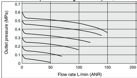
ARM5BA-307 (One-touch fittings: IN \phi 6 , OUT \phi 4 ) Condition: Inlet pressure 0.7 MPa
