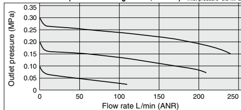
ARM5AA1-310-1 (One-touch fittings: IN \phi 8, OUT \phi 6) Condition: Inlet pressure 0.5 MPa
