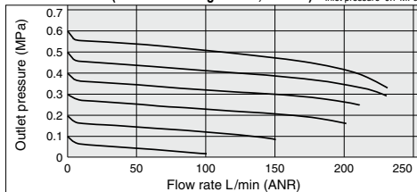
ARM5AA1-310 (One-touch fittings: IN \phi 8, OUT \phi 6) Condition: Inlet pressure 0.7 MPa
