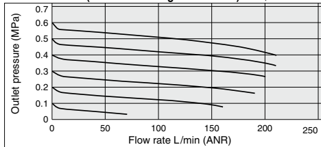
ARM5AA1-309 (One-touch fittings: IN \phi 8, OUT \phi 4) Condition: Inlet pressure 0.7 MPa
