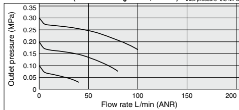
ARM5AA1-308-1 (One-touch fittings: IN/OUT \phi 6) Condition: Inlet pressure 0.5 MPa
