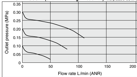
ARM5BA-307-1 (One-touch fittings: IN \phi 6 , OUT \phi 4 ) Condition: Inlet pressure 0.5 MPa
