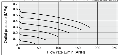
ARM5AA1-308 (One-touch fittings: IN/OUT \phi 6) Condition: Inlet pressure 0.7 MPa
